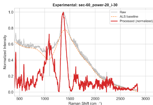
Figure 4.16: Optimized experimental Raman spectrum of Lipopolysaccharide (LPS).
