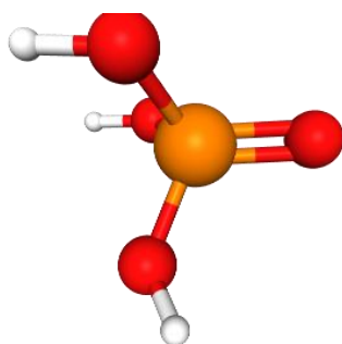
Phosphoric Acid
